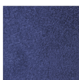
INDIGO 4359
